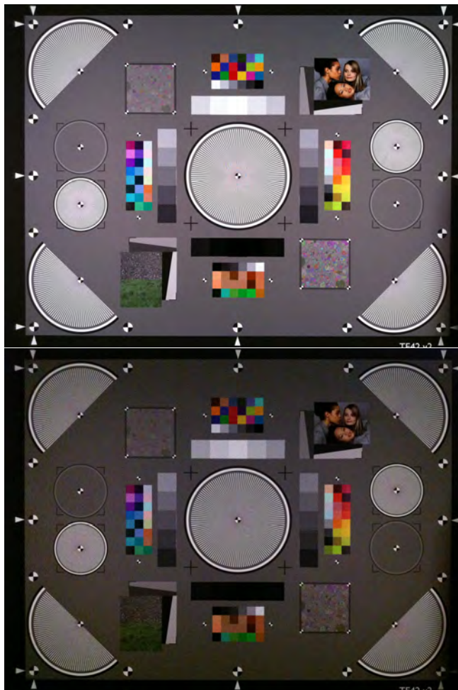
Figure 4: The upper image of the iphone 4 as captured with an illumination level of 100lx and the lower with one of 12 lx. The exposure time is limited to 1/15 sec. and making the image brighter would amplify the noise even more.
