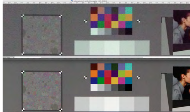
Figure 1: The upper image under low light (64 lx) is noisier, shows less detail and has a stronger a color shading than the lower image that was captured under bright light (1000 lx).
